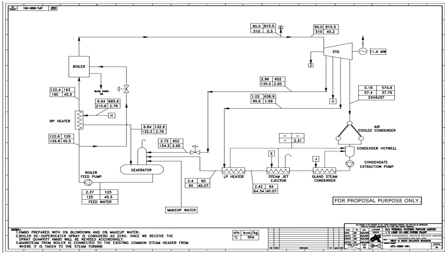
Heat and Mass Balance Diagram
