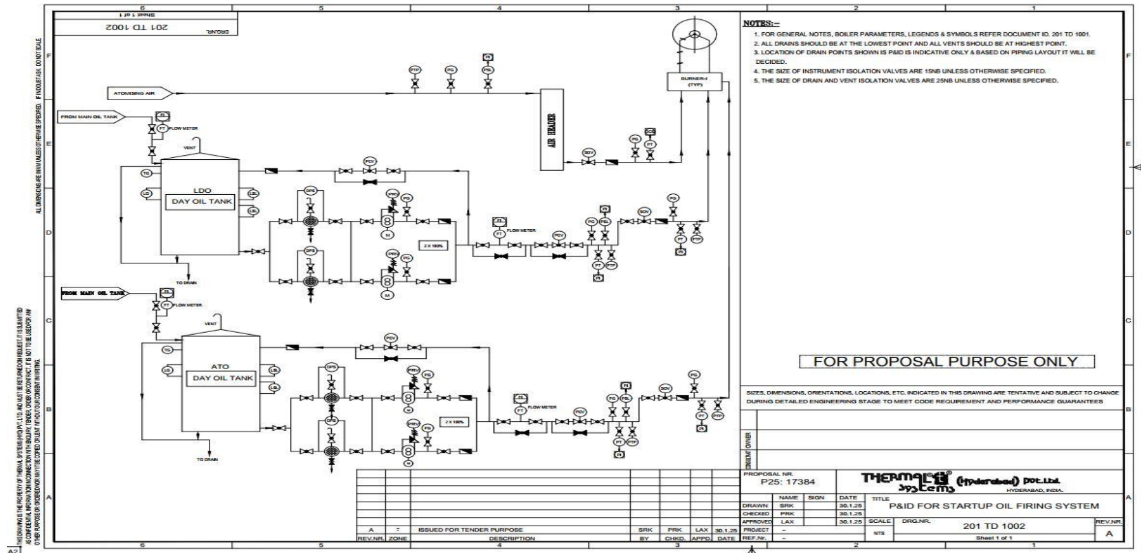
P&ID of Startup Oil Firing
